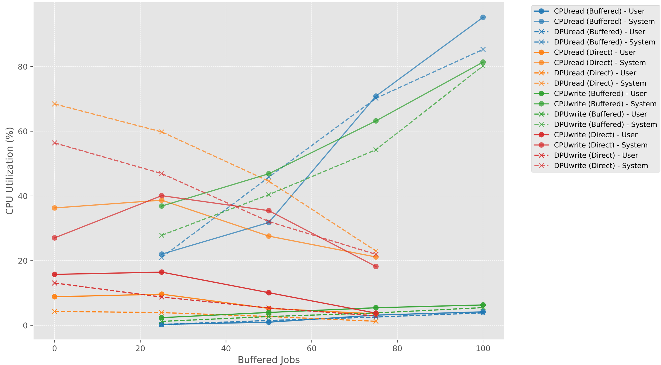
CPU Utilization vs Buffered Jobs (mixed) - SEQ (CPU vs DPU)
